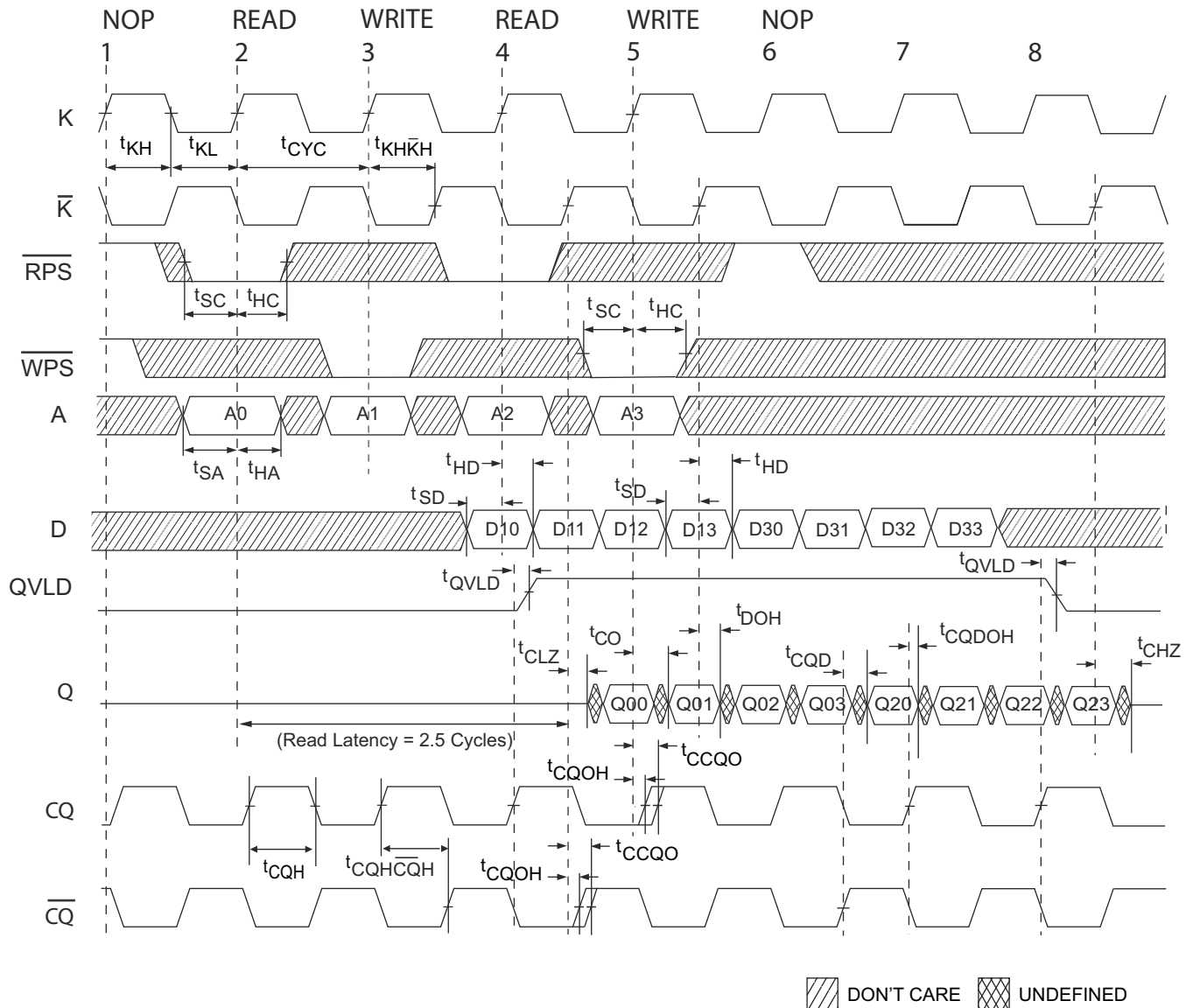
Figure 5. Waveform for 2.5-Cycle Read Latency [42, 43, 44]
