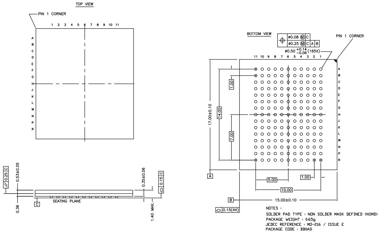
Figure 6. 165-ball FBGA (15 × 17 × 1.40 mm) (0.50 Ball Diameter) Package Outline, 51-85195
