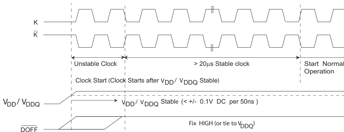
Figure 3. Power-Up Waveforms
