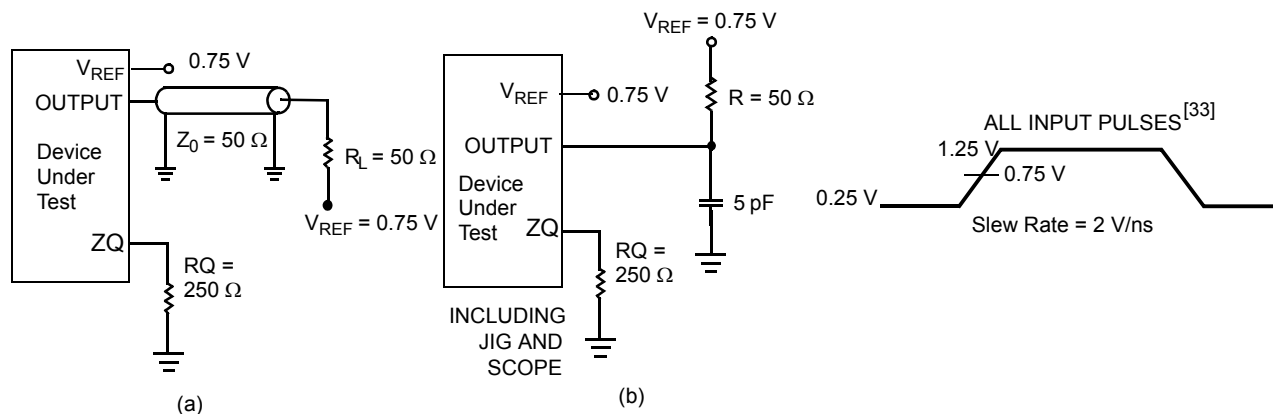
Figure 4. AC Test Loads and Waveforms
